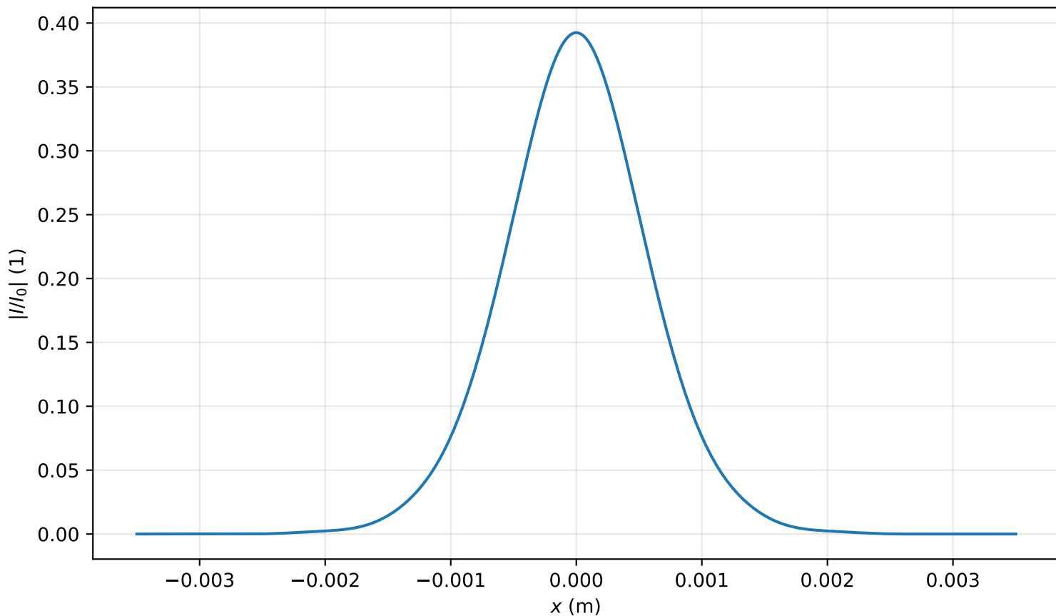
Intensity profile I(x, y = 0, z = 3.981m)/I_0 , P_{in}=0.5P_{cr} , artificial time
